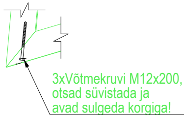
DETAIL C 1:20
