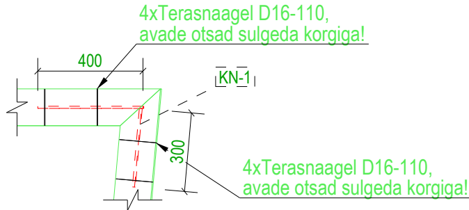
DETAIL B 1:20
